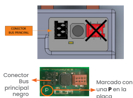
Figura 11: Detalle conector negro del bus principal
