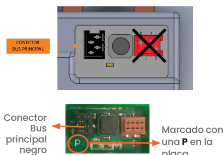
Figura 11: Detalle conector negro del bus principal
