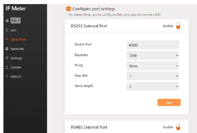
Figura 14 Web server – Serial Ports
